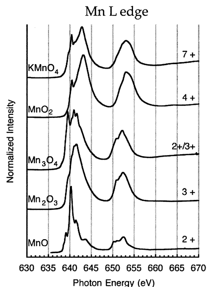
Figure 1. Manganese L edge X-ray absorption spectra of the samples given in Table 1. The formal Mn oxidation states are given on the right.
